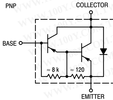
Figure 12. Darlington Schematic
