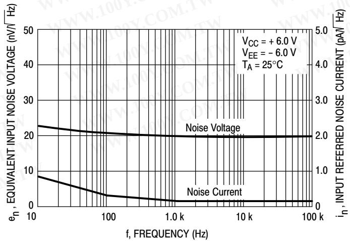
Figure 25. Equivalent Input Noise Voltage and Current versus Frequency
