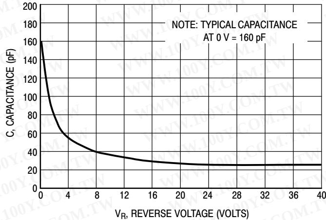
Figure 3. Typical Capacitance
