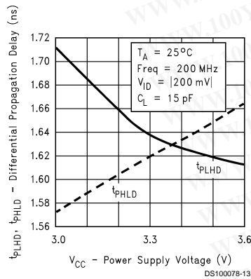
Differential Propagation Delay vs Power Supply Voltage
