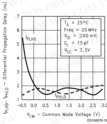
Differential Propagation Delay vs Common-Mode Voltage
