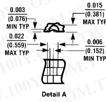
Ceramic Leadless Chip Carrier (E) Order Number 54LS14MQB NS Package Number E20A
