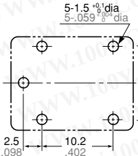
PC board pattern (Bottom view)
