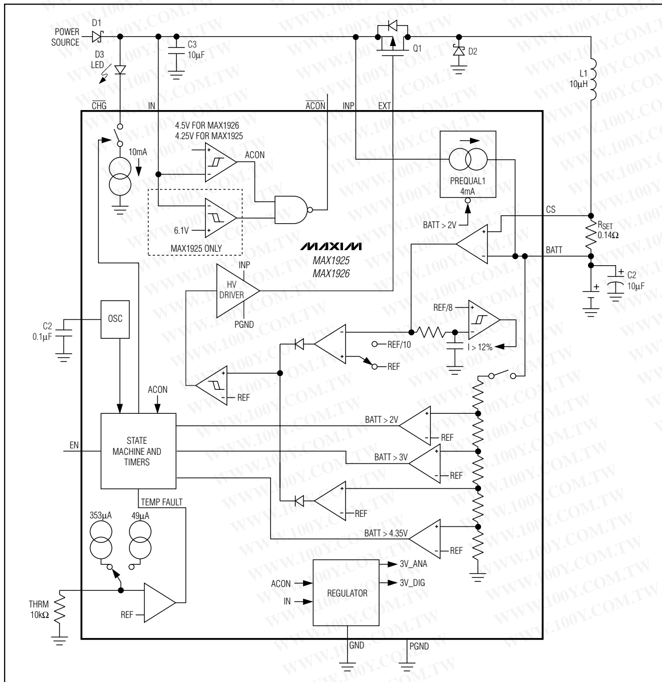
Figure 1. Functional Diagram
