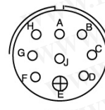
22-17 8-#16,1-#12 D(A),BAL=A
