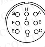
22-20 9-#16 A
