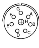
18-8 7-#16,1-#12 A
