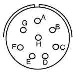
20-7 8-#16 D(A,B,G,H)A(C,D,E,F)
