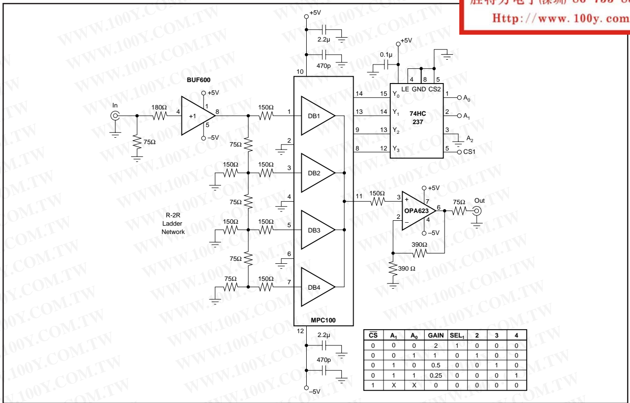
FIGURE 7. Digital Gain Control.
