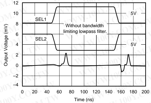
SWITCHING TRANSIENTS (Channel To Channel)
