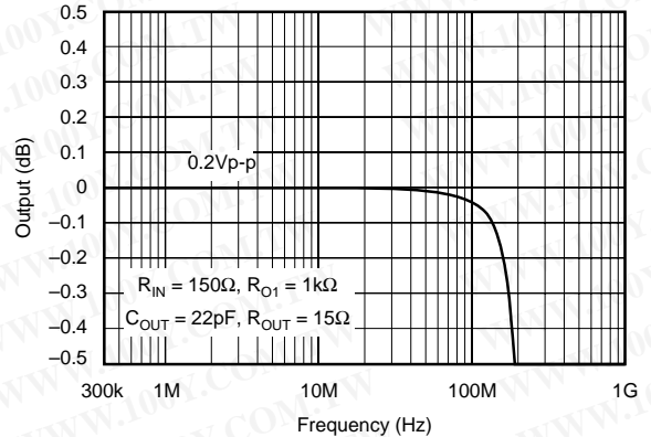
GAIN FLATNESS
