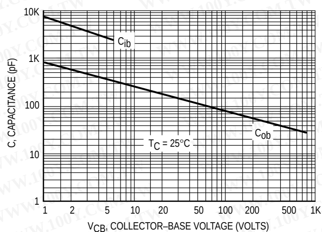
Figure 6. Typical Capacitance
