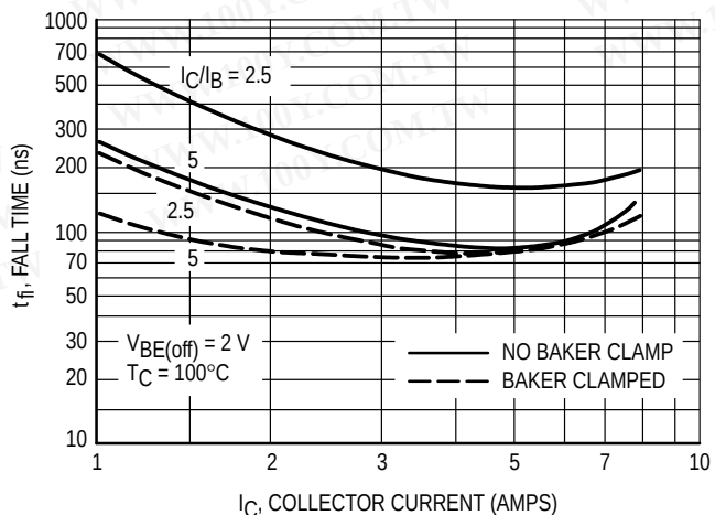
Figure 8. Inductive Switching Fall Time
