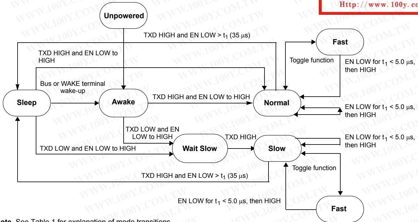
Figure 13. Mode Transitions
