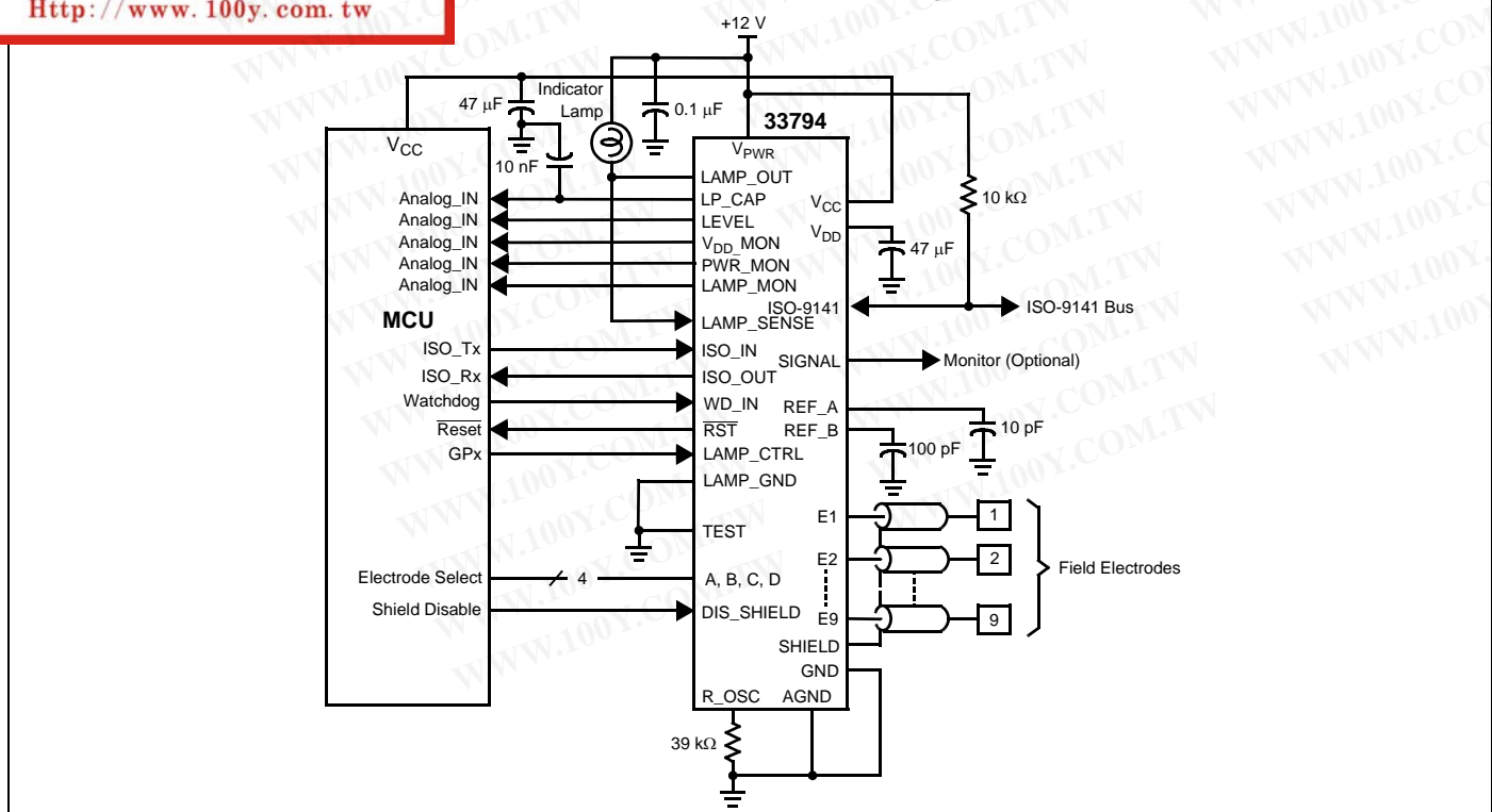
33794 Simplified Application Diagram
