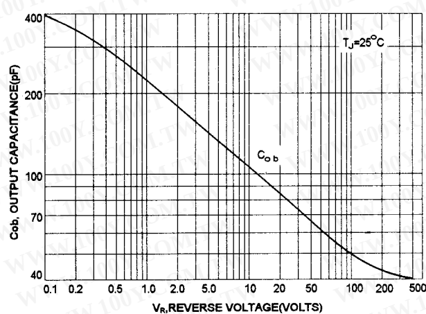
OUTPUT CAPACITANCES
