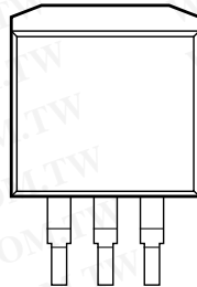
INPUT GROUND OUTPUT TO-263 Package (MIC2940A-xxBU)
