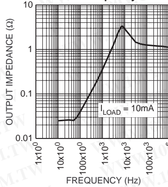
Output Impedance vs. Frequency
