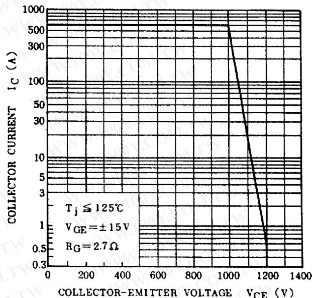
REVERSE BIAS SOA
