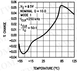
fCLK/fo Deviation vs Temperature
