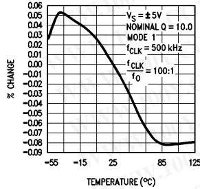
fCLK/fo Deviation vs Temperature
