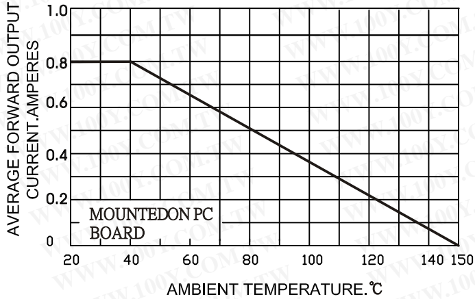
FIG.1-DERATING CURVE FOR OUTPUT RECTIFIER CURRENT
