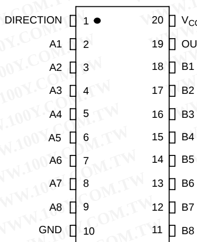
Figure 1. Pin Assignment
