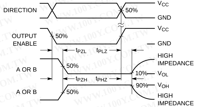
Figure 4. Switching Waveform
