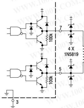
Figure 19. Enhanced System Performance with Common Switching Regulators
