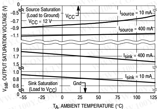
Figure 11. Drive Output Saturation Voltage versus Temperature
