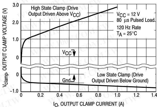
Figure 9. Drive Output Clamp Voltage versus Clamp Current
