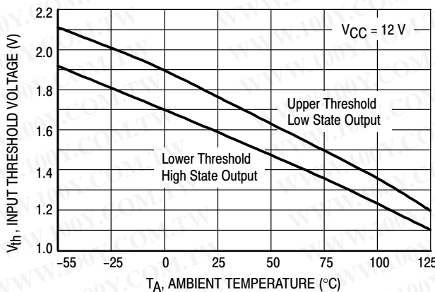
Figure 5. Logic Input Threshold Voltage versus Temperature
