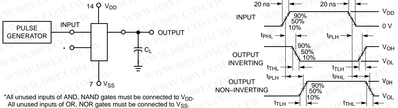
Figure 3. Switching Time Test Circuit and Waveforms
