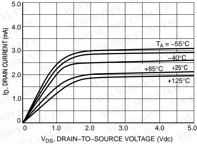
Figure 5. V_{GS} = 5.0 Vdc
