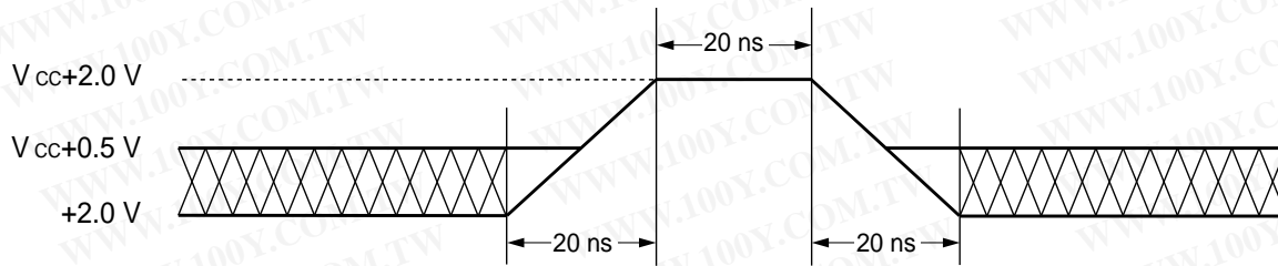
Figure 2 Maximum Positive Overshoot Waveform
