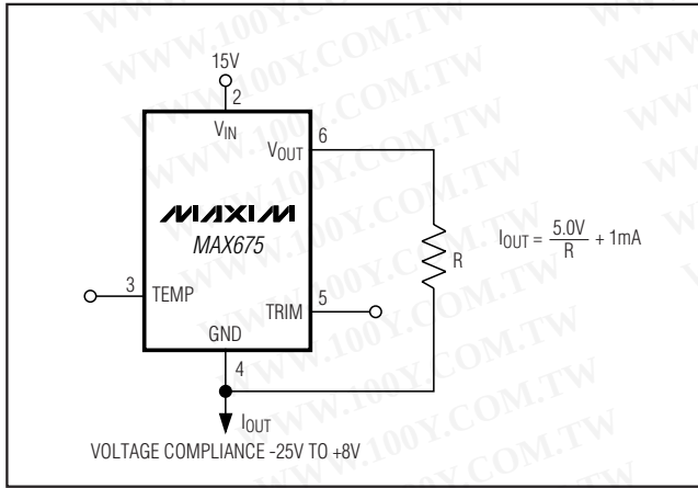
Figure 5. Current Source
