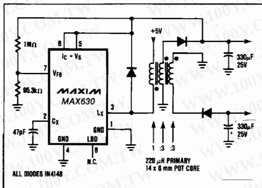
Figure 3. +5V to \pm 15 V Converter
