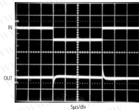
LINE-TRANSIENT RESPONSE
