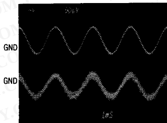
REFERENCE FEEDTHROUGH AT 400Hz
