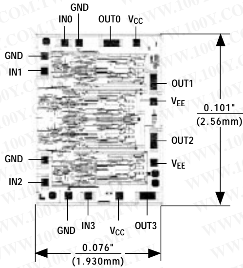
Chip Topography
