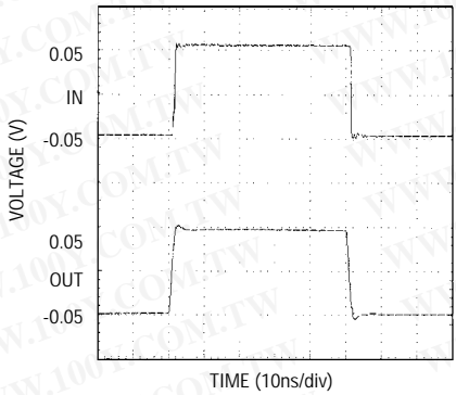
MAX496 SMALL-SIGNAL PULSE RESPONSE
