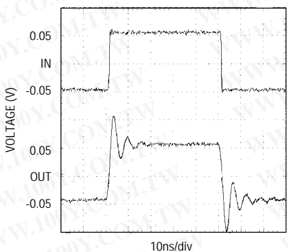
MAX496 SMALL-SIGNAL PULSE RESPONSE ( C_L = 47pF )
