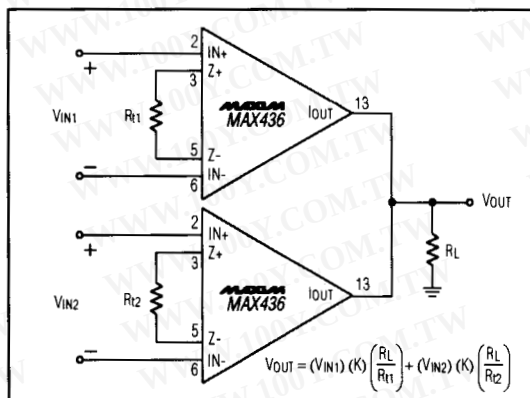
Figure 7. Summing Amplifier
