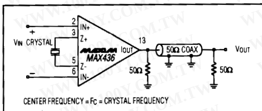
Figure 16. Crystal Tuned Amplifier
