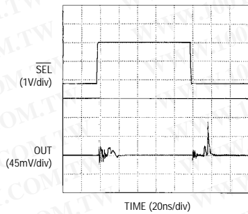
DIGITAL FEEDTHROUGH
