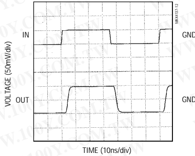
MAX4137 SMALL-SIGNAL PULSE RESPONSE ( A_{VCL} = +2 )
