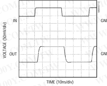
MAX4138 SMALL-SIGNAL PULSE RESPONSE ( A_{VCL} = +2 )
