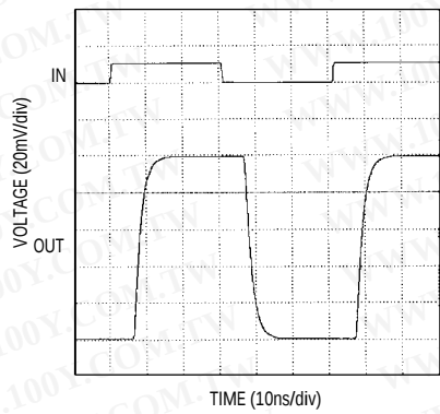
MAX4112/MAX4117/MAX4119 SMALL-SIGNAL PULSE RESPONSE ( A_{VCL} = +10 )
