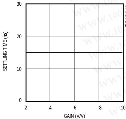
MAX4112/MAX4117/MAX4119 SETTLING TIME vs. GAIN
