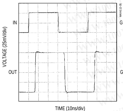
MAX4112/MAX4117/MAX4119 SMALL-SIGNAL PULSE RESPONSE ( A_{VCL} = +2 )
