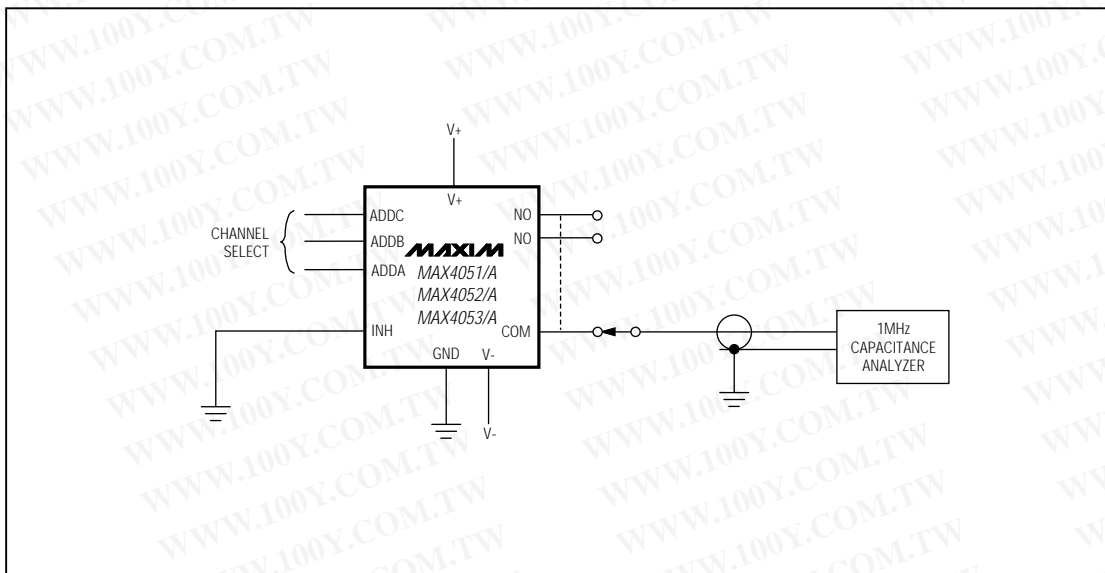
Figure 7. NO/COM Capacitance
