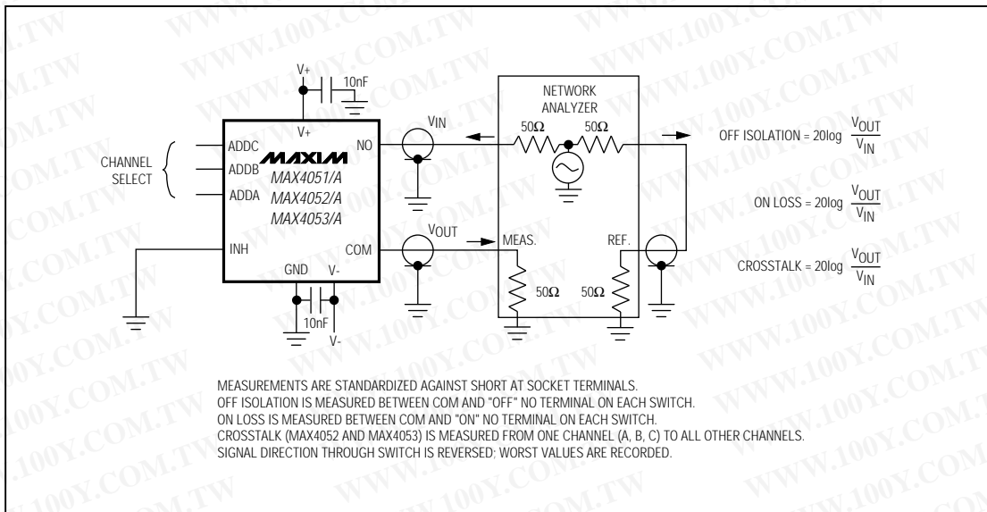
Figure 6. Off Isolation, On Loss, and Crosstalk
