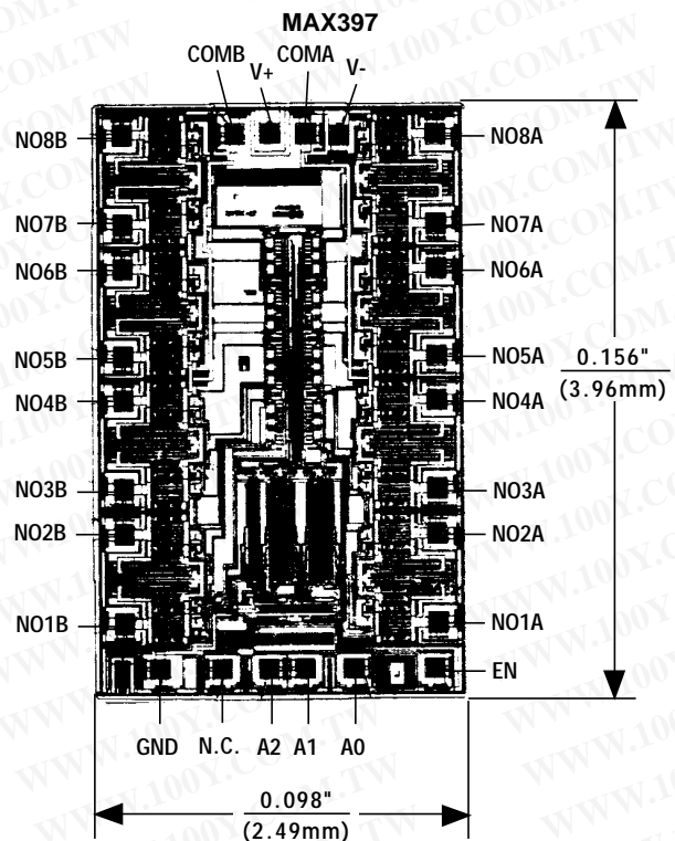
TRANSISTOR COUNT: 360 SUBSTRATE CONNECTED TO V+
