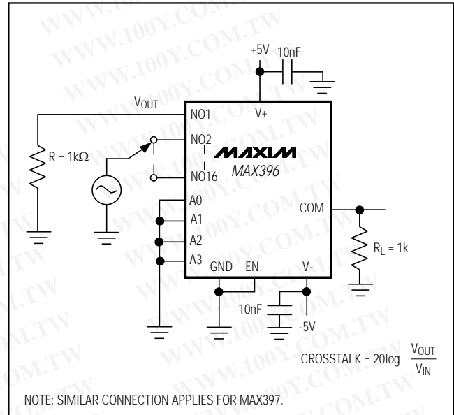
Figure 7. Crosstalk ( V_{CT} )
