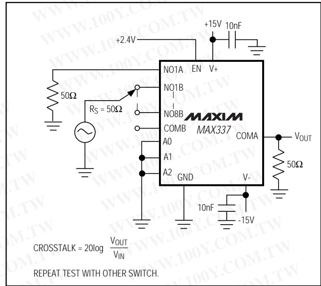
Figure 7. Crosstalk
