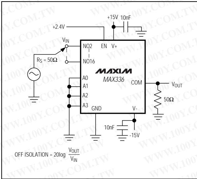
Figure 6. Off Isolation
