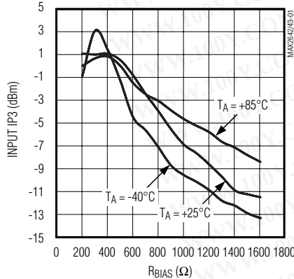
INPUT THIRD-ORDER INTERCEPT vs. R_{BIAS} (HIGH GAIN)
