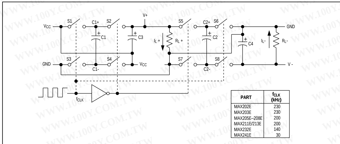
Figure 4. Charge-Pump Diagram
