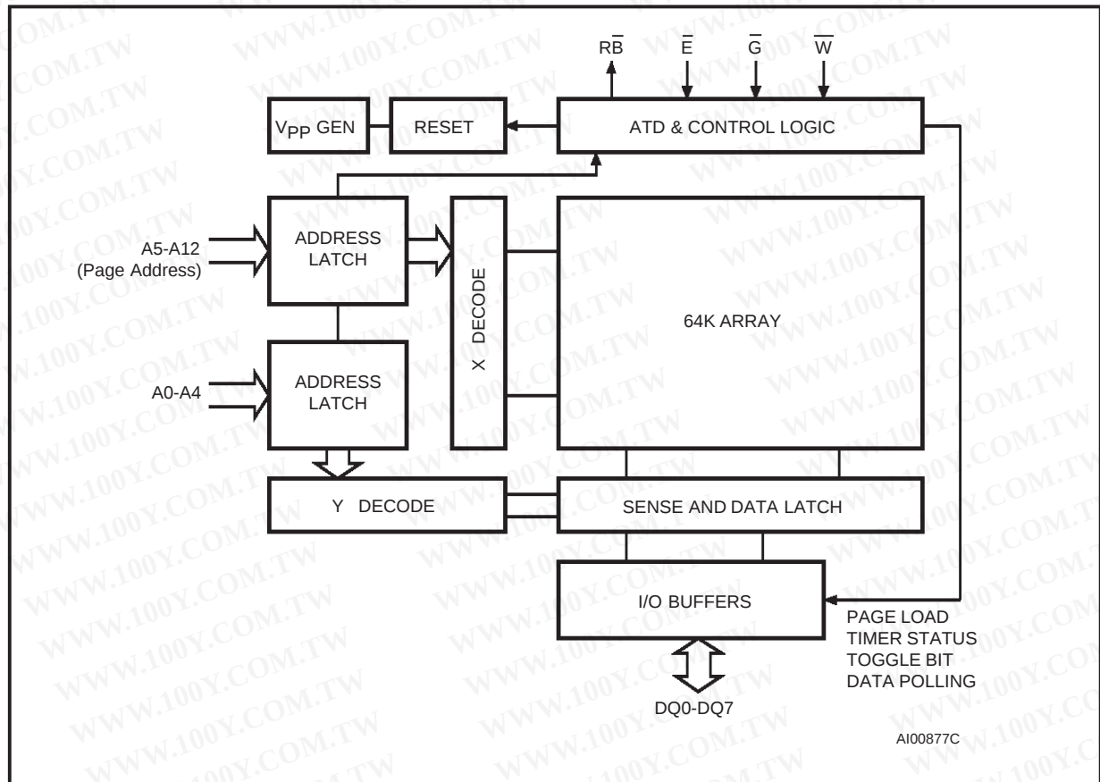
Figure 3. Block Diagram
