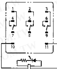
AC Model
