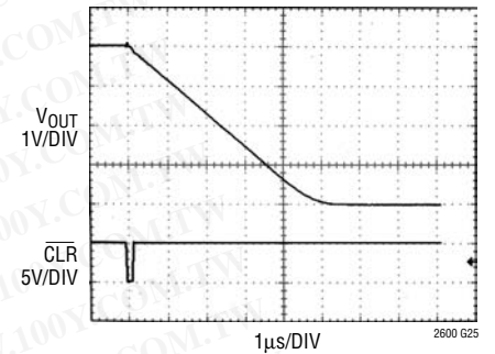
Hardware CLR
