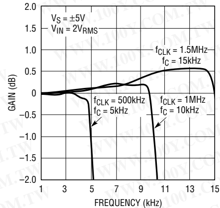
Passband Gain vs Clock Frequency, V_S = \pm 5\text{V}
