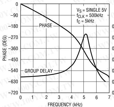
Phase and Group Delay vs Frequency
