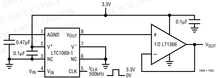
Single 3.3V Supply Operation with Output Buffer
