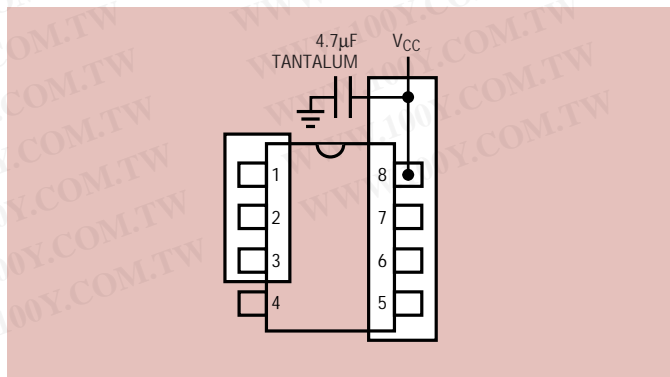
Figure 4. Example Ground Plane for the LTC1091
