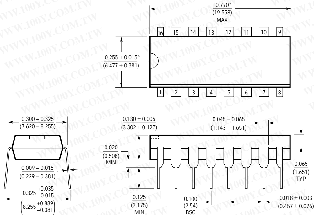
N Package 16-Lead PDIP (Narrow 0.300) (LTC DWG # 05-08-1510)
