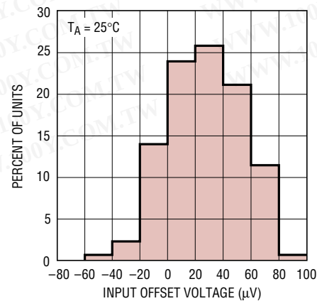
Distribution of Offset Voltage at V_S = \pm 1.0\text{V} (In All Packages)
