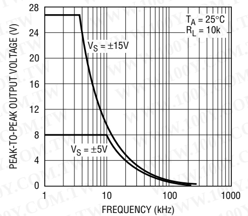
Undistorted Output Voltage vs Frequency
