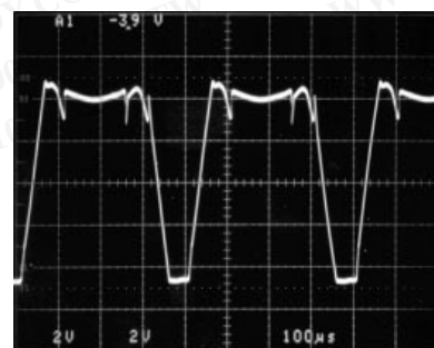
OP-297 Output
