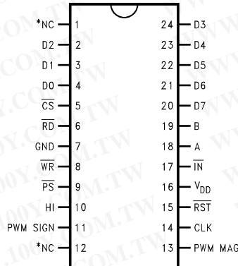
Figure 4. LM629M
