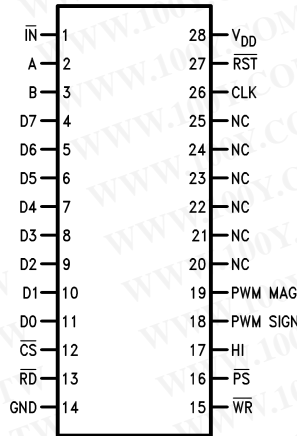
Figure 4. LM629M
