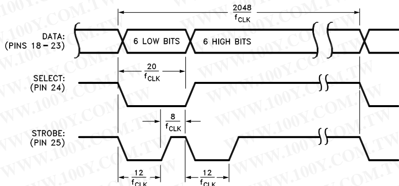
Figure 11. 12-Bit Multiplexed Output Timing
