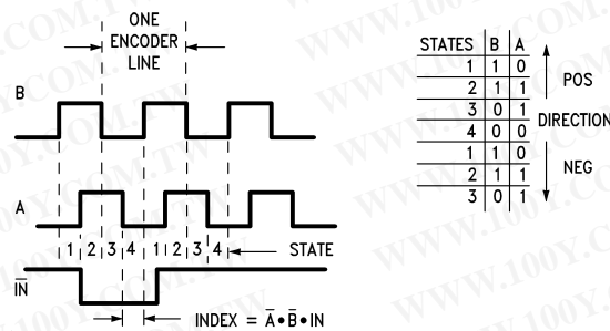
Figure 12. Quadrature Encoder Signals
