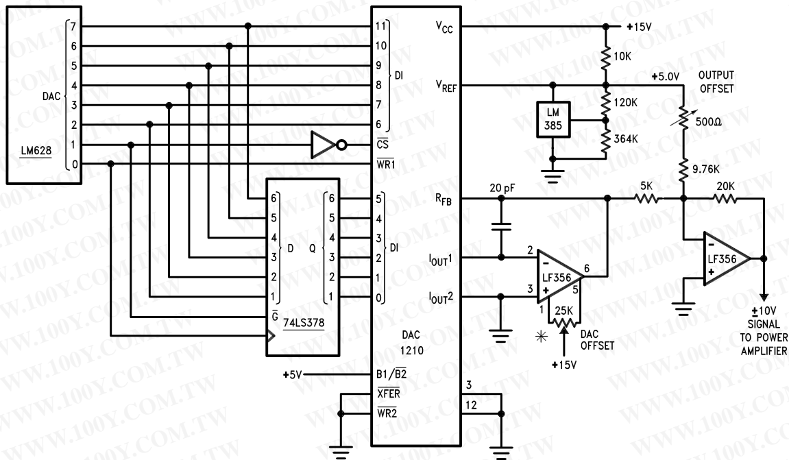
Figure 17. Interfacing a 12-Bit DAC and LM628
