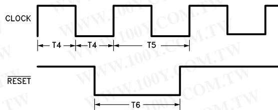
Figure 6. Clock and Reset Timing
