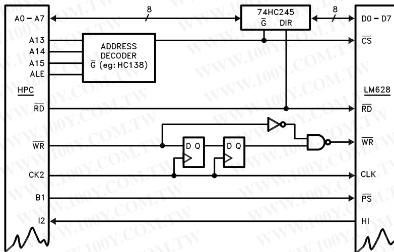
Figure 16. LM628 and HPC Interface
