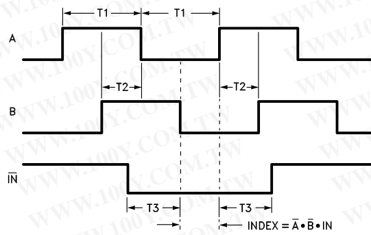
Figure 5. Quadrature Encoder Input Timing
