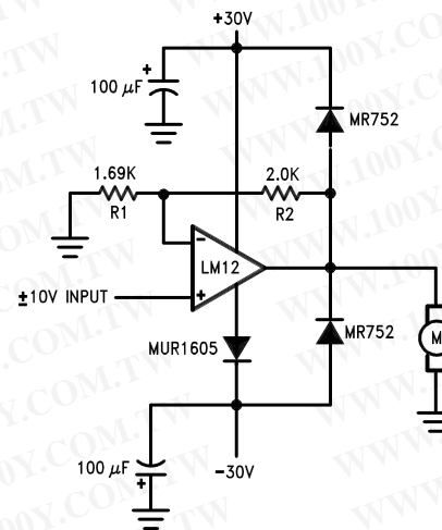
Figure 18. Driving a Motor with the LM12 Power Op Amp
