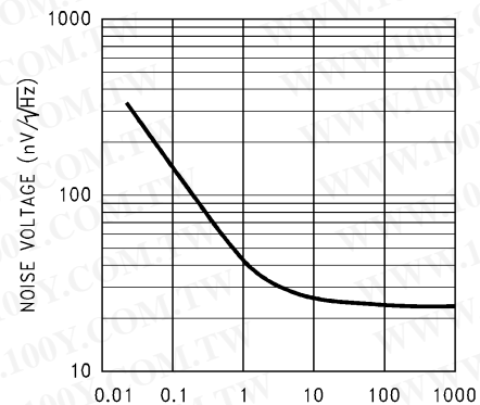
Noise Voltage vs. Frequency
