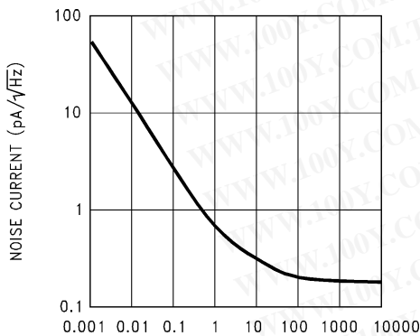
Noise Current vs. Frequency
