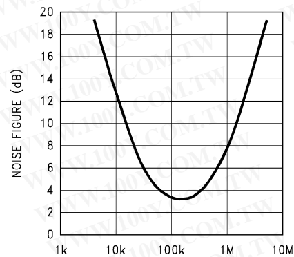
NF vs. Source Resistance
