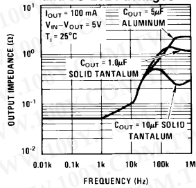
Output Impedance TO-5 and TO-202 Packages
