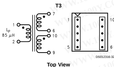
FIGURE 17. Coilcraft Q4343-B
