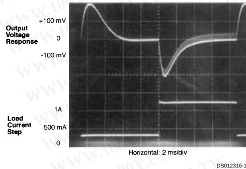
FIGURE 6. V_{OUT} Load Current Step Response
