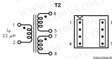
FIGURE 16. Coilcraft Q4337-B
