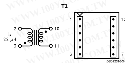
FIGURE 19. Coilcraft Q4435-B (Surface Mount)
