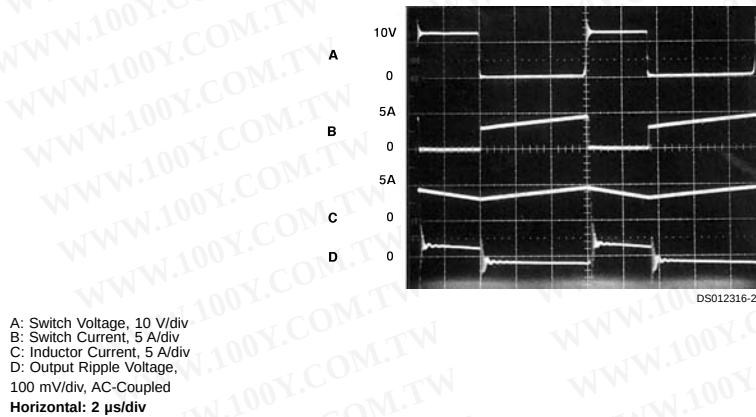
FIGURE 34. Switching Waveforms
