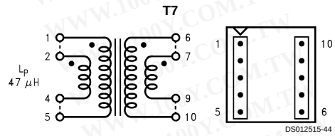
Top View FIGURE 27. Schott 26606
