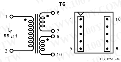
Top View FIGURE 28. Schott 67140900
