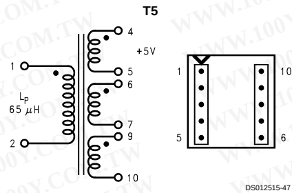
Top View FIGURE 29. Schott 67140890
