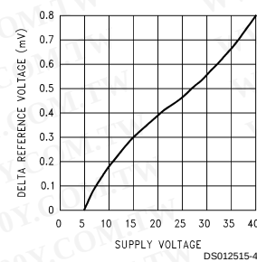
\Delta Reference Voltage vs Supply Voltage
