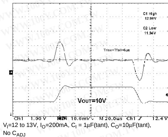
Figure 26: Line Transient
