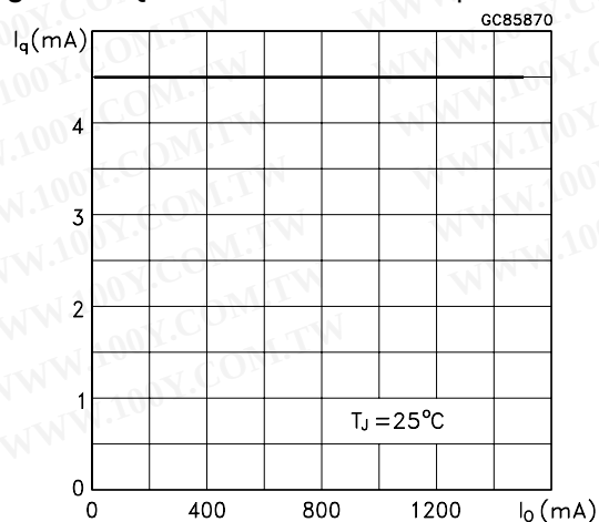
Figure 15: Quiescent Current vs Output Current
