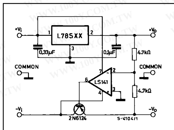
Figure 20 : Tracking Voltage Regulator.
