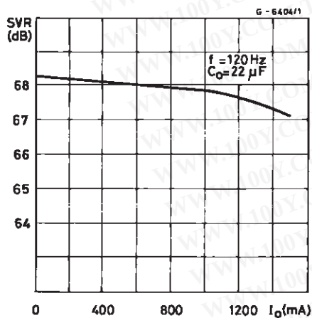
Figure 20 : Supply Voltage Rejection vs. output Current.
