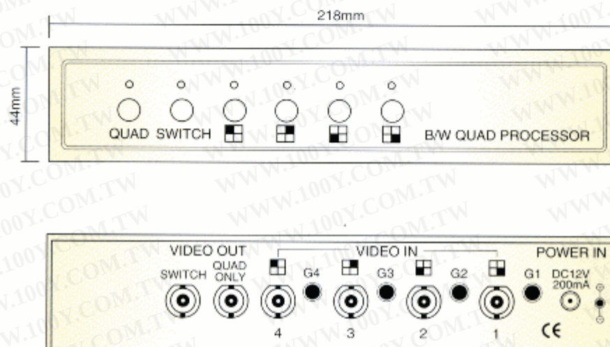
Rear Panel
