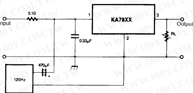
Figure 7. Ripple Rejection
